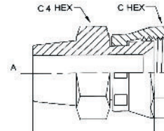
PART NO. TUBE O.D. A Weld B FJS 37Deg B DRILL L1 LGTH L LGTH C HEX C4 HEX
