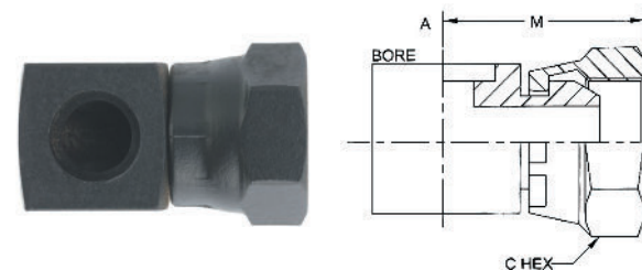
PART NO. TUBE O.D. A BORE A1 NPSM M LGTH C HEX
