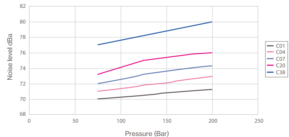
Noise @ maximum displacement, 1500 rpm measured 1 m from rear of pump. Fluid viscosity 20cSt, fluid density 880 3 Kg/m (includes background noise 56 dBa)
